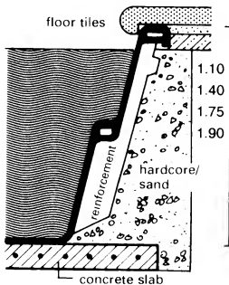
⑨ Polyester prefabricated pool
